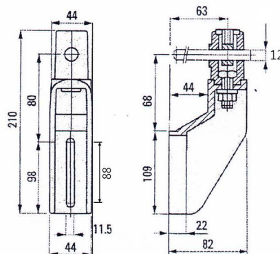
■ MIT-SB021 Adjustable bracket
