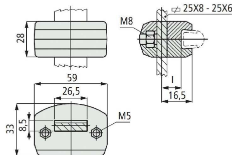
■ A222-001 Adjustable guide rail clamp
