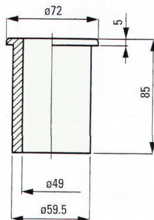
■ MIT-FS324 Threaded bushings for round tubes
