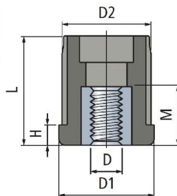
■ MIT-FS224 Threaded bushings for square tubes
