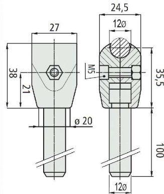
■ MIT-CL770 Double guide rail clamp
