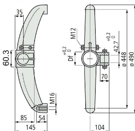
■ 616-624552 Support Base (bipod 120°)( \phi 60.3 \sim \phi 42.7 )
