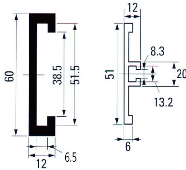
■ MIT-GL001 Aluminum guide+C profile (3M/支)
