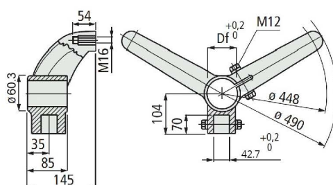
■ 616-624552 Support Base (bipod 120°)( \phi 60.3 \sim \phi 42.7 )
