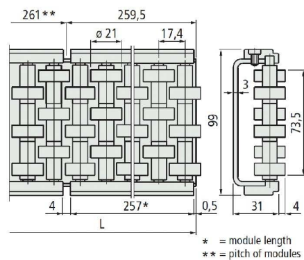
■ 128-62660 Guide rail for accumulation
