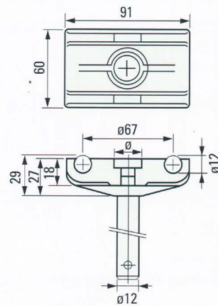
■ MIT-CL159 Adjustable guide rail clamp
