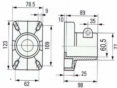
■ MIT-FS740 Frame Support
