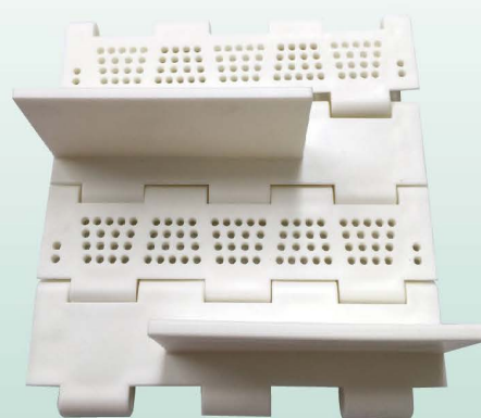
STW-381-PP+檔板H=50
