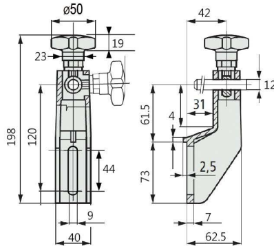
■ MIT-SB639 Middle side guide bracket
