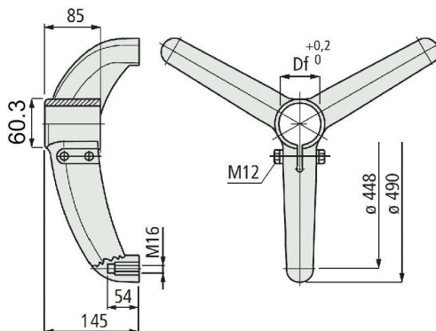
■ MIT-615 Support Base (tripod)( \phi 60.3 )
