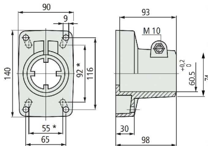
■ MIT-124-6197 \phi 48.3 / MIT-152404 \phi 50 Reduction bushing
