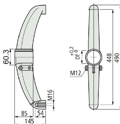
■ MIT-619 Support Base (bipod 180°)( \phi 60.3 \sim \phi 42.7 )
