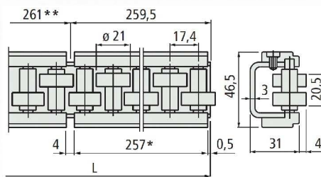
■ 128-62640 Guide rail for accumulation
