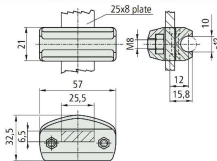
■ MIT-CL159 Adjustable guide rail clamp
