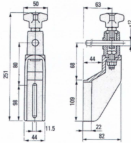
■ MIT-SB022 Adjustable bracket
